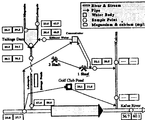
Figure 8. Magnesium & Calcium contents (mg/l) in surface (October 1992).
