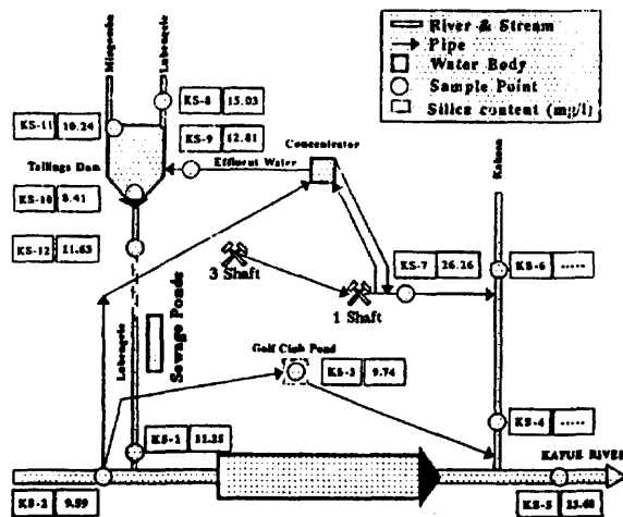
Figure 9. Silica contents (mg/l) in surface water (October 1992)
