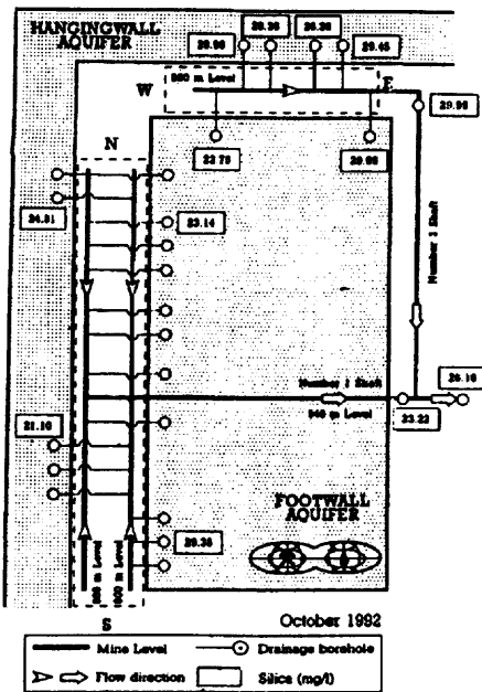
Figure 14. Silica Contents (mg/l) in groundwater (October 1992).
