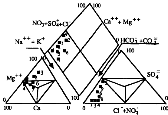
Figure 6. Piper diagram including all the surface water analysis (October 1992)
