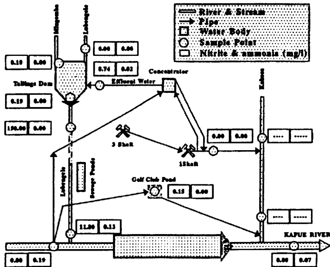
Figure 7. Nitrite & Ammonia contents (mg/l) in surface water (October 1992).
