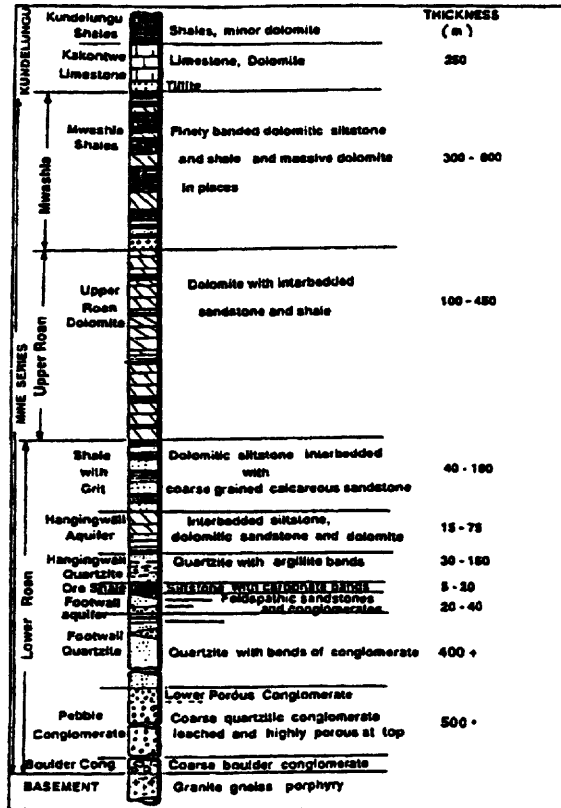
Figure 3. Konkola Mine stratigraphic column (Mulenga 1991).
