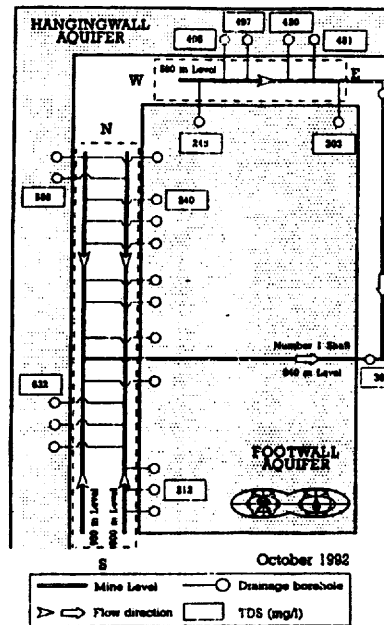
Figure 15. Total Dissolved Solids contents (mg/l) in groundwater (October 1992).
