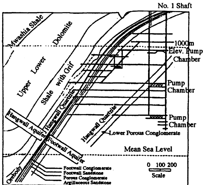
Figure 2. Generalized geological cross section at Number 1 Shaft (Mulenga, 1991).
