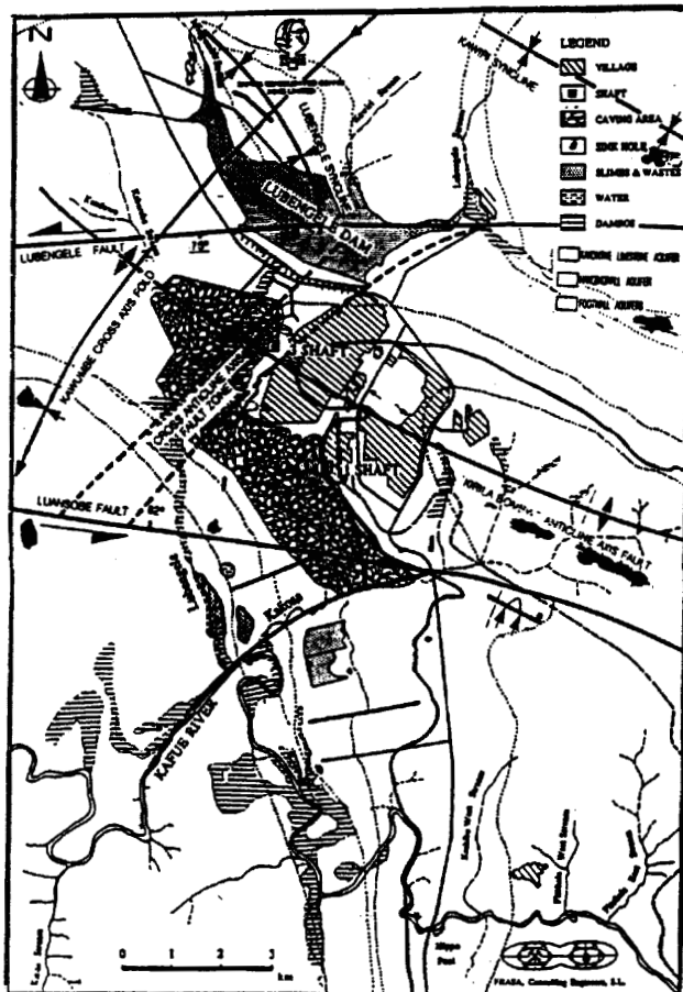
Figure 5. Simplified hydrogeological map of Konkola Mine area.
